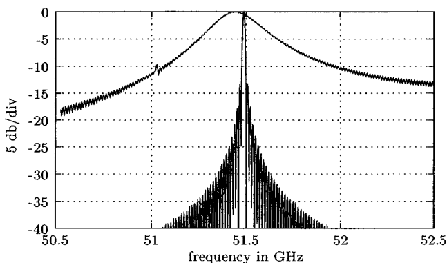
Fig. 6. Spectra around 51.5 GHz for the semi and fully implicit scheme.
