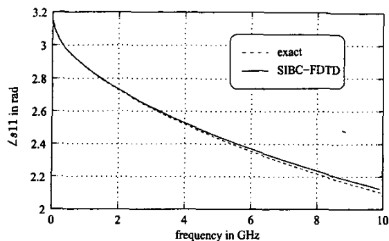
Figure 6: Scattering parameters of a symmetric three layer conductor.
