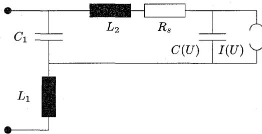
Figure 2: Equivalent circuit of the diode
