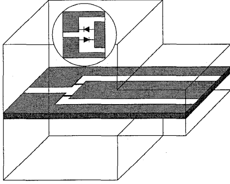
Figure 1: Basic structure of the doubler
