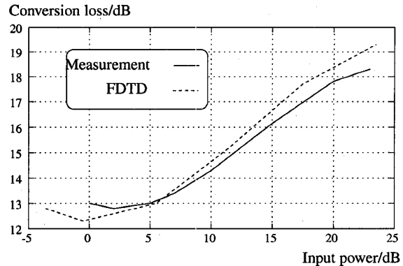
Figure 4: Conversion loss at 20 GHz
