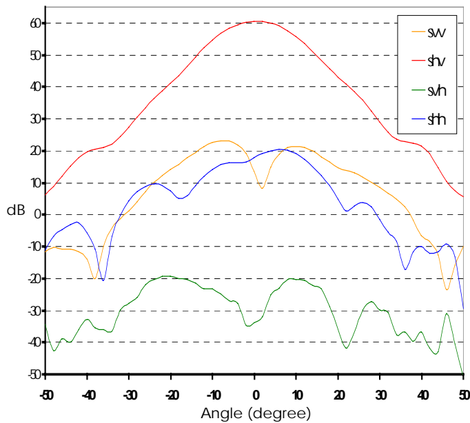
0° orientation RCS Azimuthal Patterns
