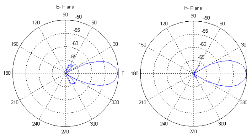
E & H Plane Beam Pattern
